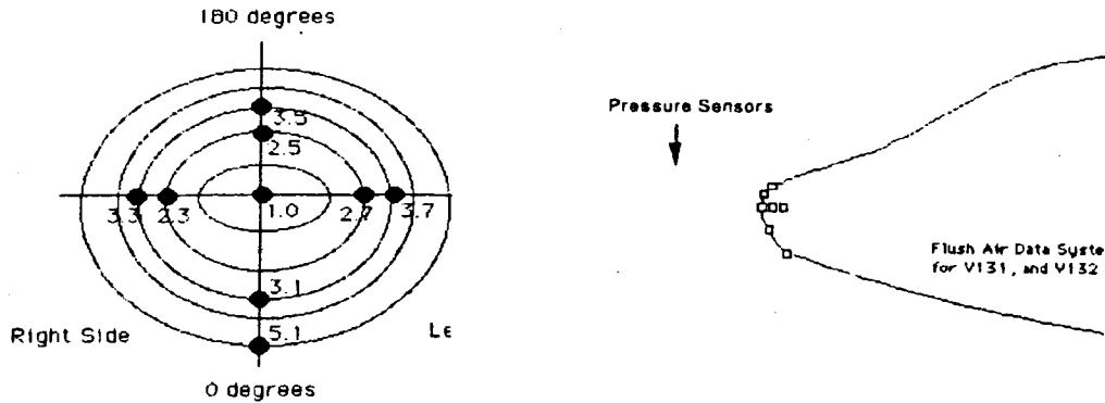
FADS nose ports looking aft
