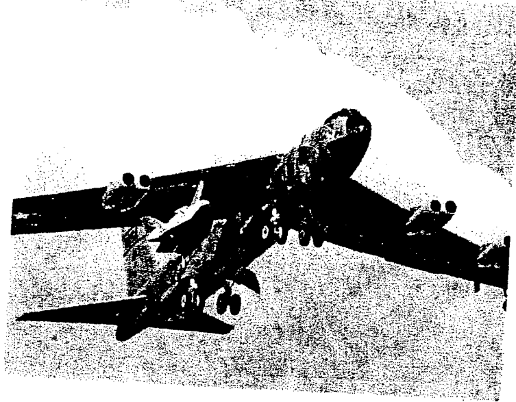
Figure 1- Photograph of X-38 V131 during captive carry flight 1. The X38 vehicle is attached to the wing of the B52 and flown around at different altitudes and velocities to collect data. To date seven captive carry flights have been performed.
