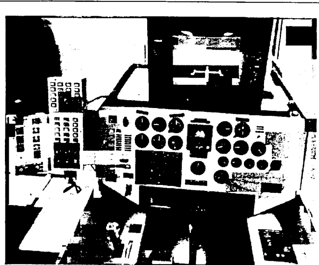
Fig. 5 HiMAT simulation cockpit.
