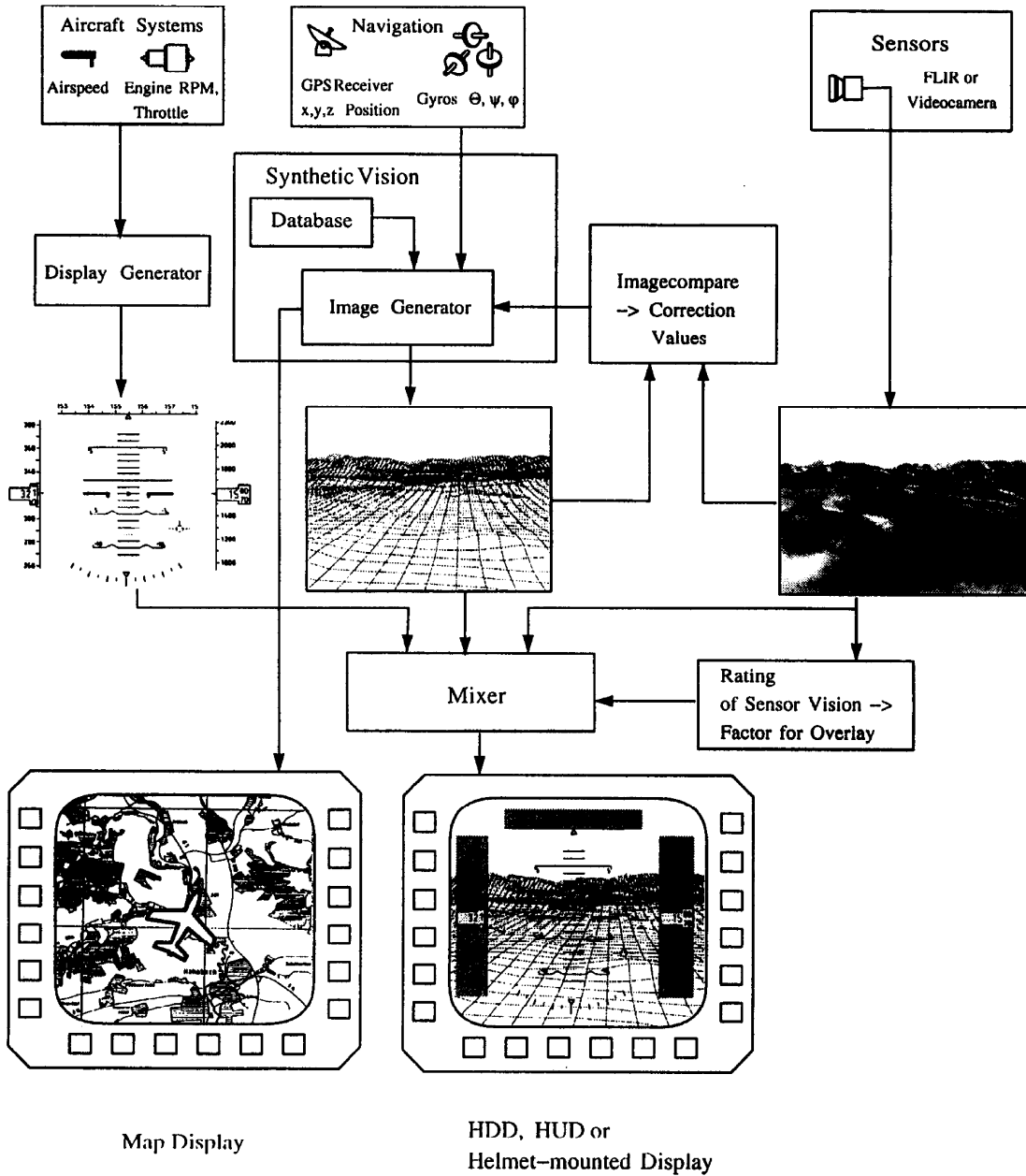
Fig. 1. System Components
